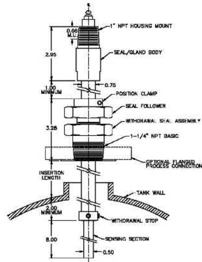
P53 Shown Top Mounted
