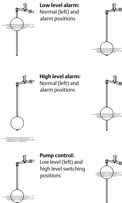
Figure 6. Pump Control and Alarm Applications
