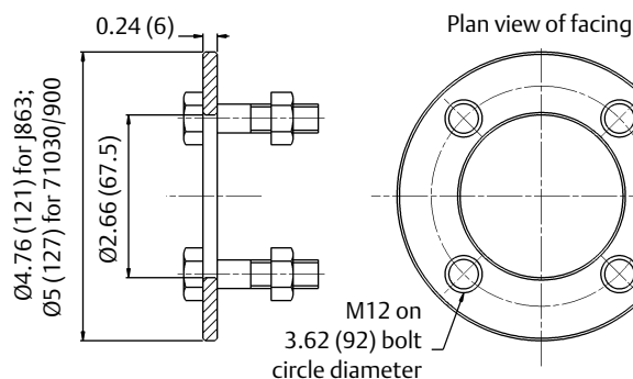
Figure 3. Companion flanges for Mobrey 'G' flanged float switches
